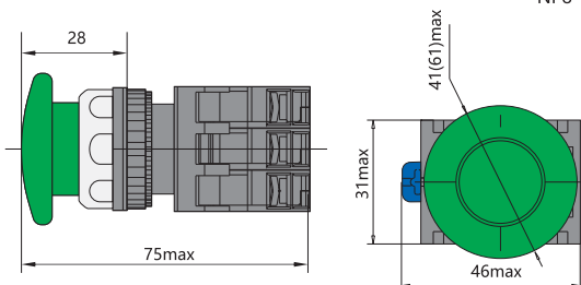
NP8-□□MD/□
