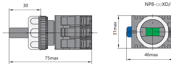
NP8-□□XD/□
