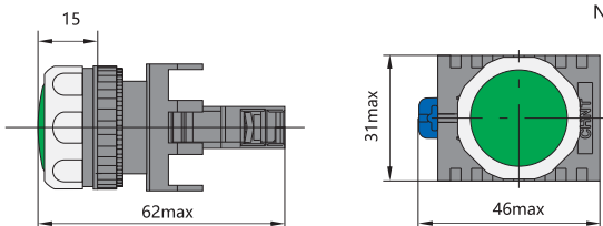
NP8-□□SD/□
