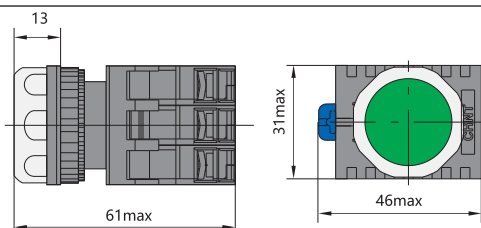
NP8-□□GND/□
