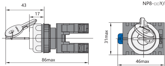
NP8-□□Y/□
